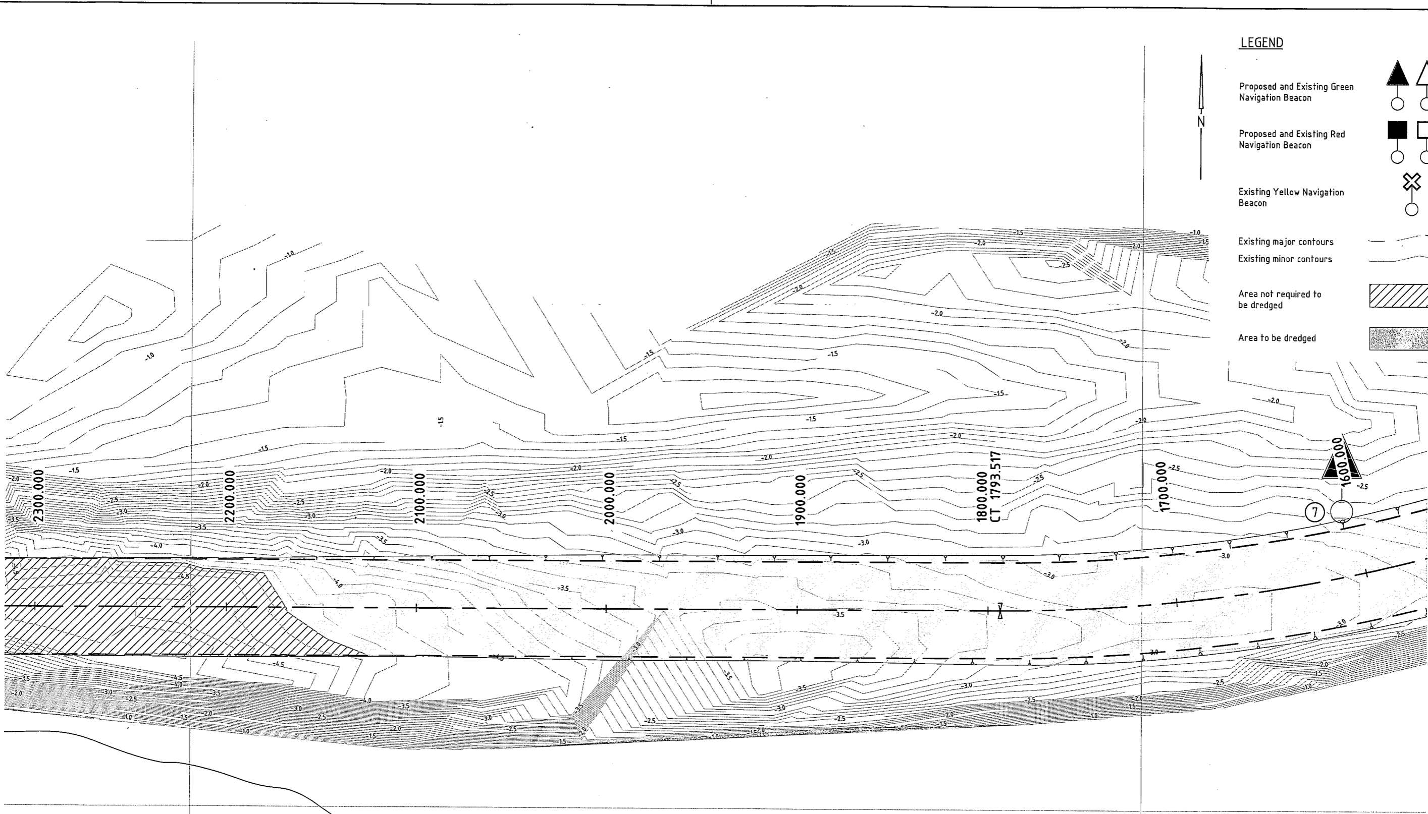
LAYOUT PLAN Scale 1:1000
